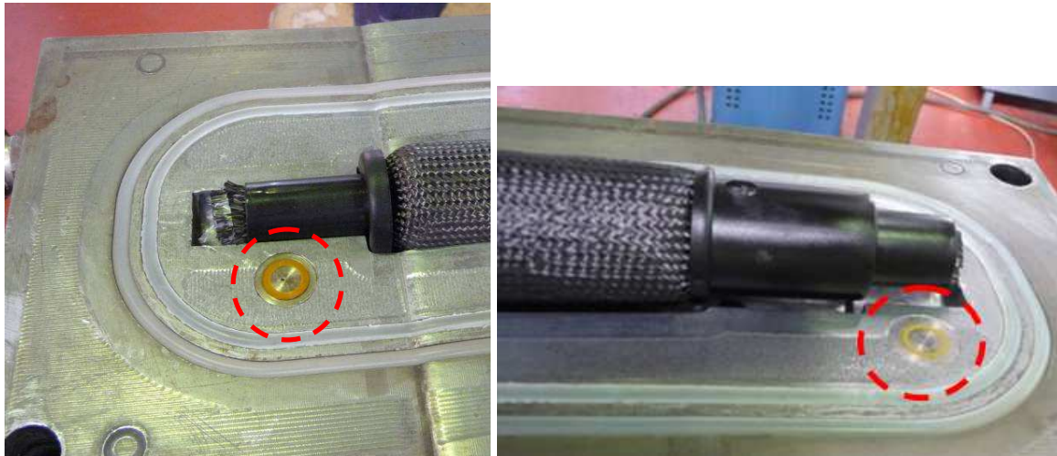
Fig.5. Flash mounted sensor at the cavity's margin near the inlet (left) and outlet (right) gates.
